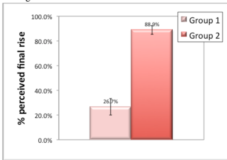
Figure 2. Percentage of perceived final rise for two groups of participants producing wh-in-situ content questions.
