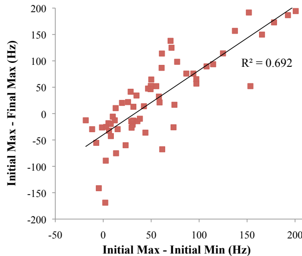
Fig. 4. Scatterplot demonstrating a correlation between two difference values for each item, based on maximal and minimal values in the wh -region and a maximal value in the sentence-final region of the wh-in-situ (content) questions.
