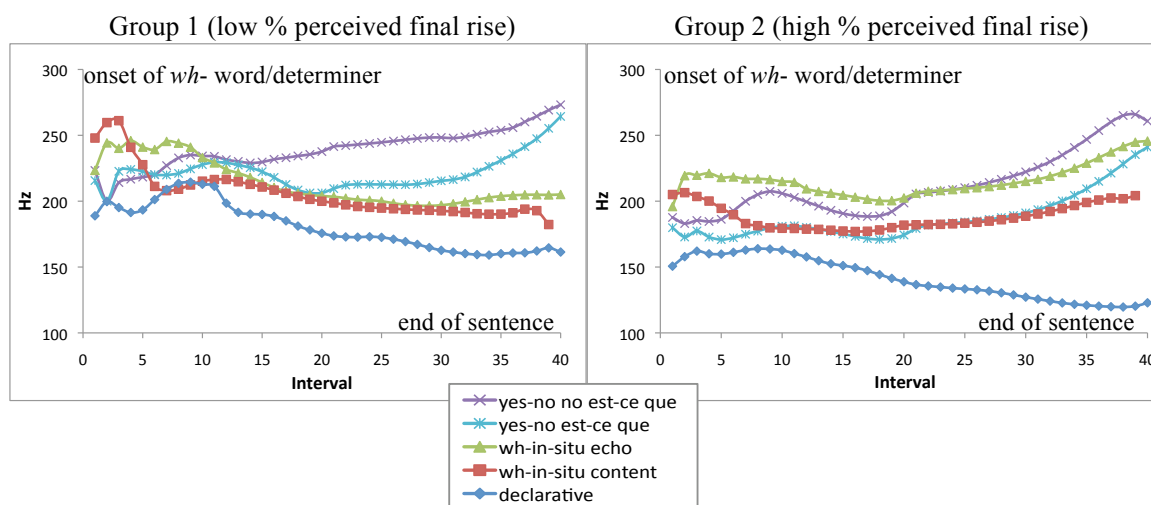
Figure 3. Sentence-final contour for five of the sentences produced by speakers in Groups 1 and 2, averaging over items and speakers.
